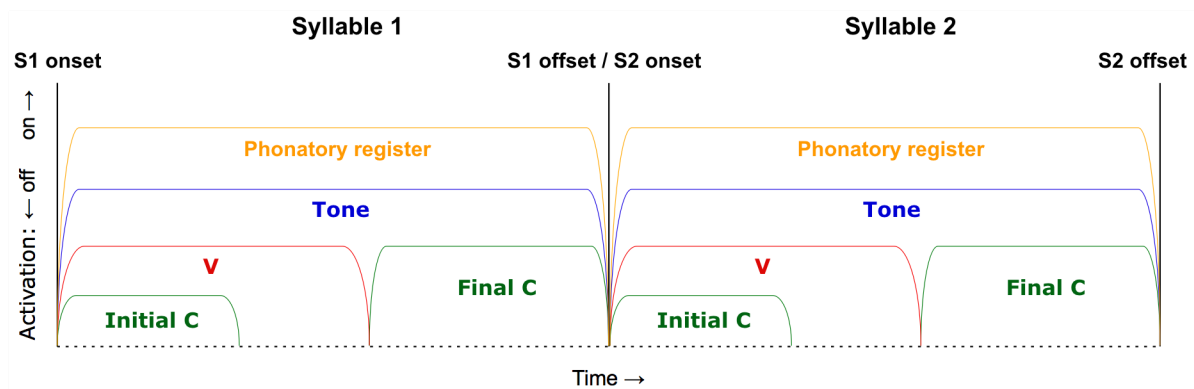
Figure 6. A simplified schematic of the time structure model.
