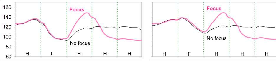
Figure 4. Mean F_0 contours of Mandarin 5-syllable utterances. Adapted from Xu (1999).
