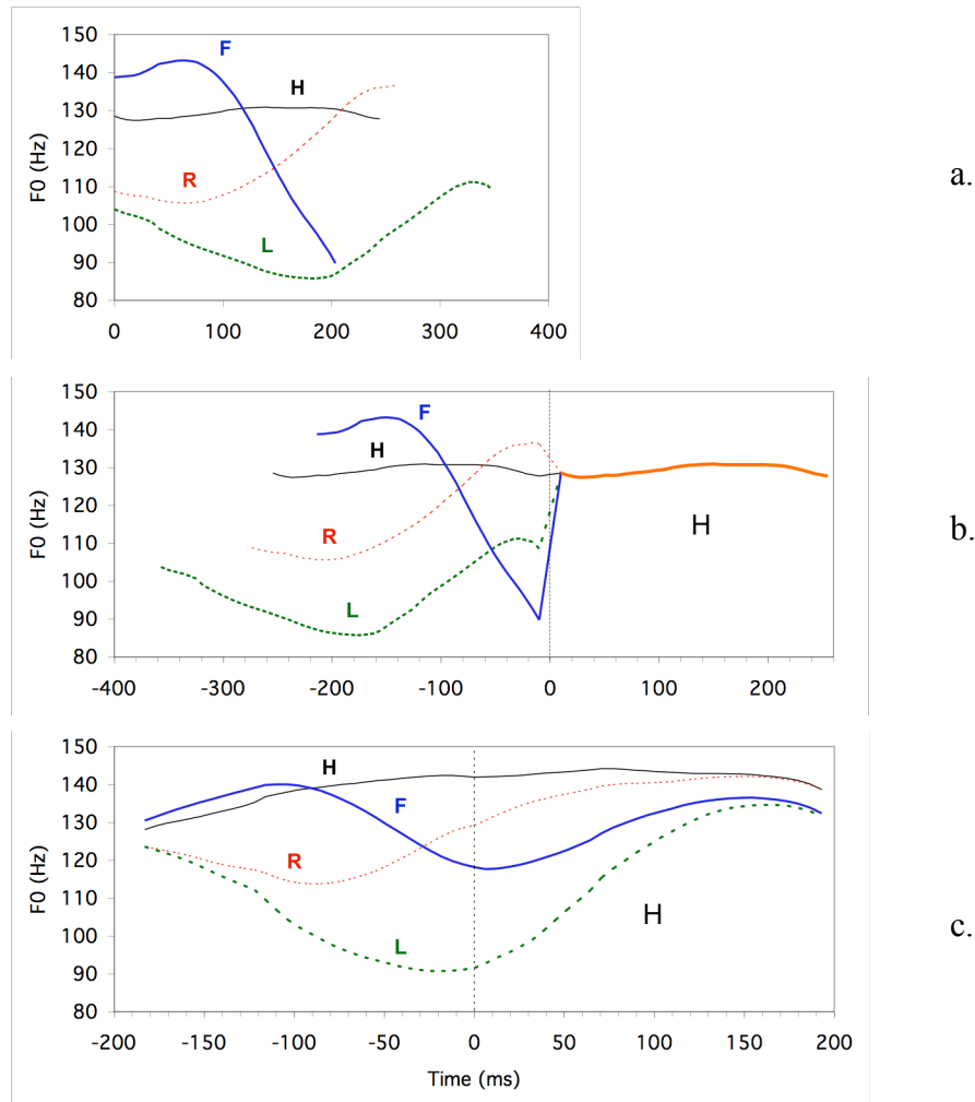
Figure 2. a. Mean F_0 contours of Mandarin tones produced in isolation. b. Isolated Mandarin H tone concatenated with different preceding tones, linked by 20 ms of arbitrary linear transition. c. Mean F_0 contours of the same two tone sequences in actual production. Adapted from (Xu, 1997)
