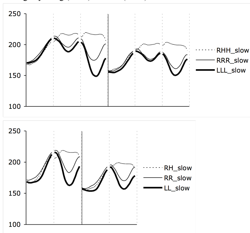
Figure 7. Overlaid mean F0 tracks of H, R and L sequences said at slow rate by all seven speakers. Each curve is a time-normalized average of 21 trials, 3 by each speaker. The averaging of F0 across all speakers in these cases is justified by the fact that LL(L) and LLL(L) were produced as RR(L) and RRR(L) by all of them.
